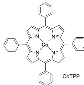
Figure 1. Structure of the cobalt(II) porphyrin (CoTPP) complex.
