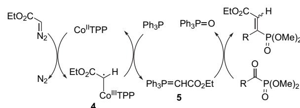
Scheme 2. Possible olefination mechanism catalyzed by CoTPP is in agreement with what is proposed in the literature. 12f
