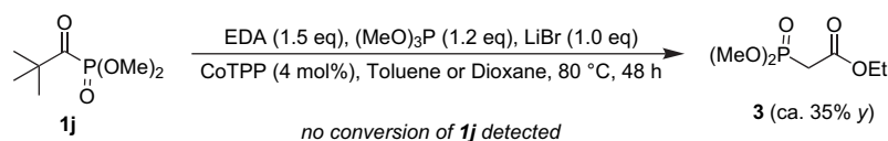
Scheme 1. Search for the olefination of 1j as the sterically hindered acyl phosphonate.
